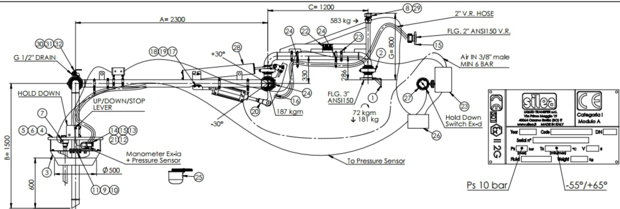
PARK POSITION + HOLES TEMPLATE
